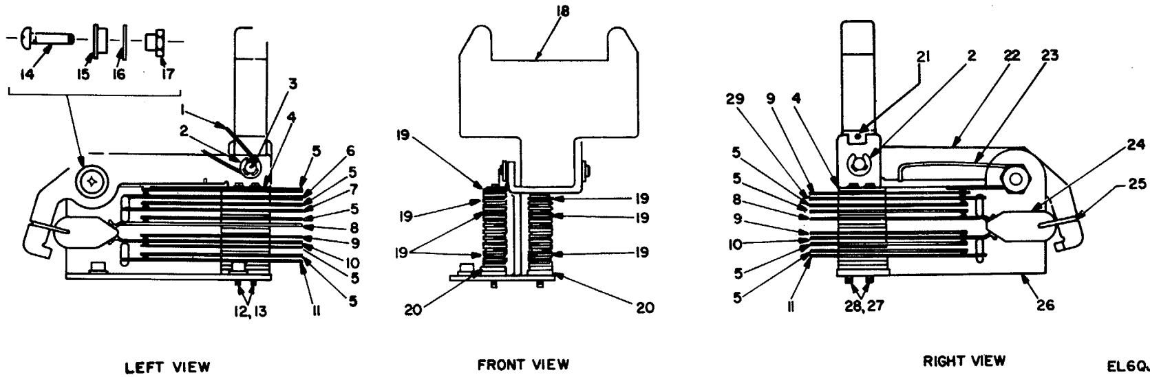
Figure 7. Hookswitch Assembly
